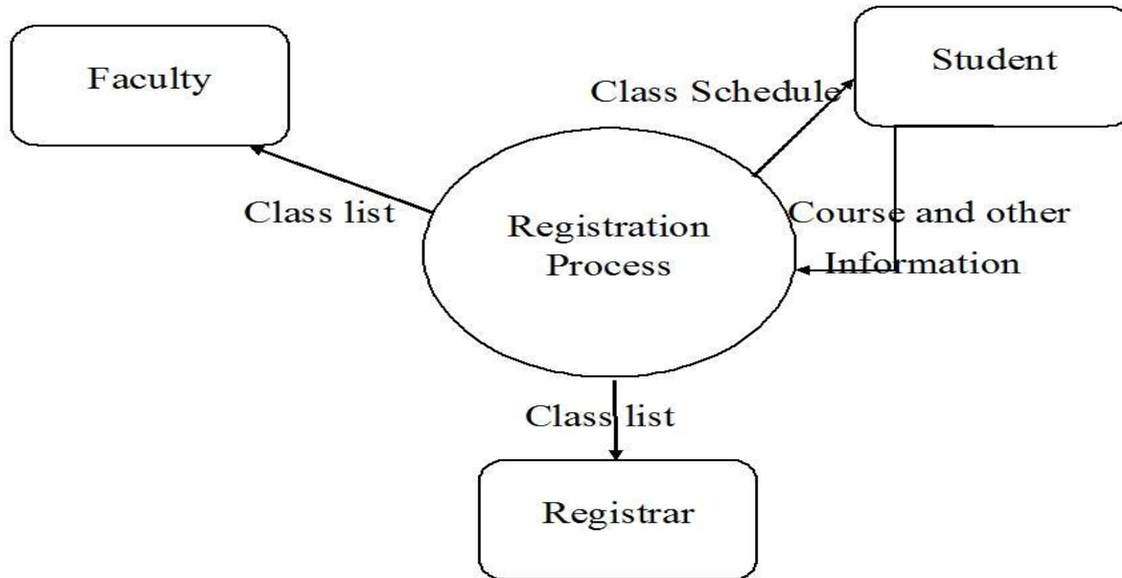
Figure: Level 0 DFD for Course Registration System
