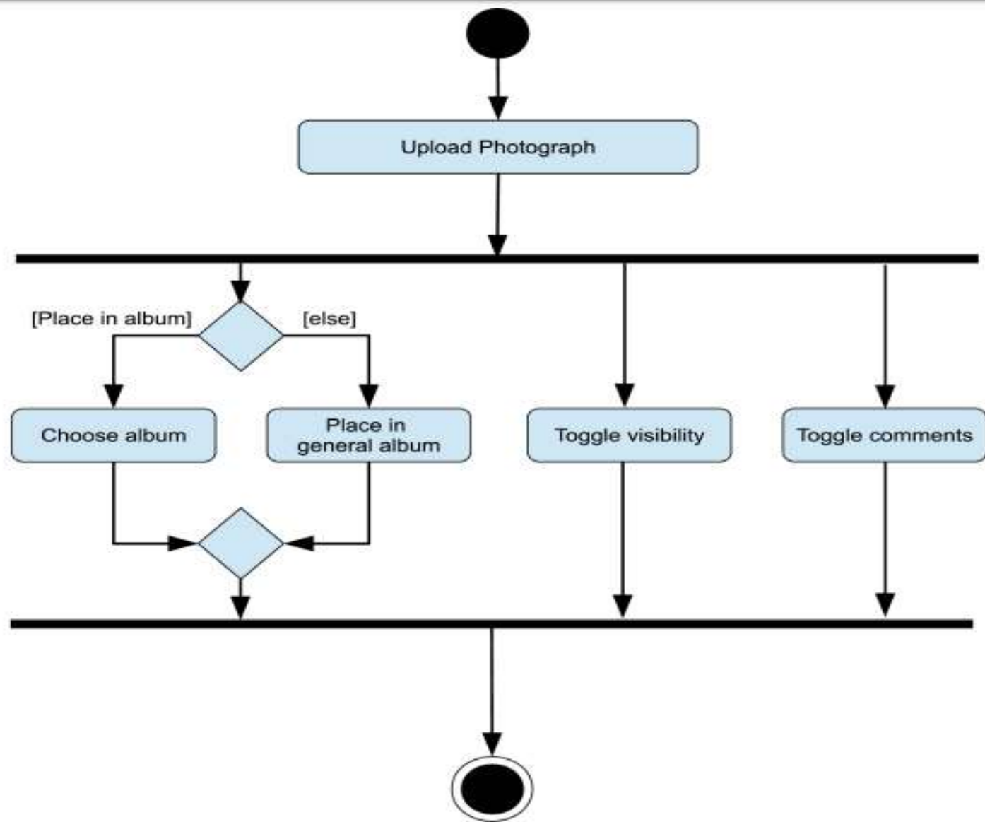
Figure: Activity Diagram Example (Without Swimlane)
